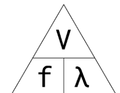
Wavelength Triangle
