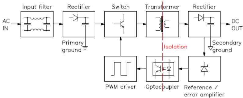
Switch mode power supply block diagram
